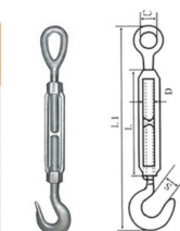
G80 Turnbuckles type OC
