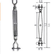
G80 Turnbuckles type UII
