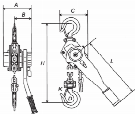
HSSH型不锈钢手扳葫芦 HSSH type stainless steel lever hoist
